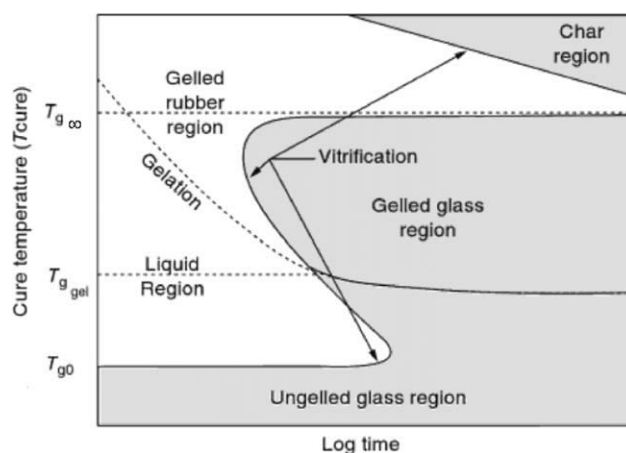
Figure 3 TTT diagram for a reactive system. 12
